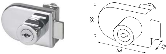
Additional Single Glass Lock 5mm 5mm 139 gr | Finishing .09
