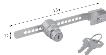
16 LOCKING POSITIONS Lock for 5mm Glass Sliding Door 78 gr | Finishing .09
