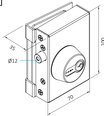
Additional Lock [Double Locking]
