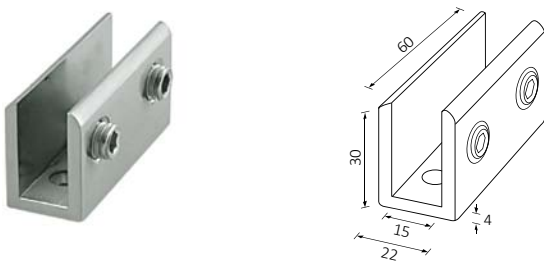
Rectangular Support 60mm
