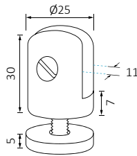
Glass-Self Support with End Stop \varnothing 25 \times 35
