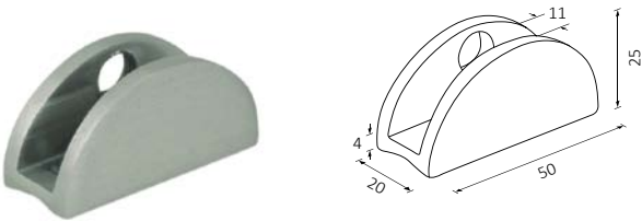
Support [Half Moon] 50mm
