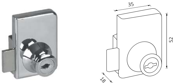
Additional Double Glass Lock 5mm 5mm 116 gr | Finishing .09
