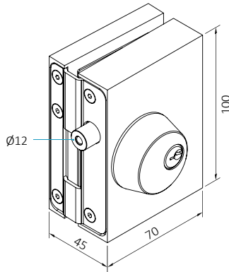
Additional Lock [Double Locking]
