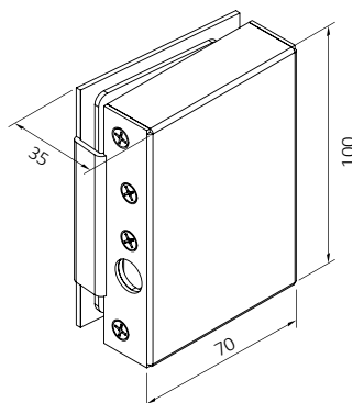
Additional Lock Female [for lock 201 Stainless Steel]
