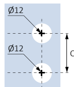
Stainless steel Handle H Ø18 Finishing .13 .14
