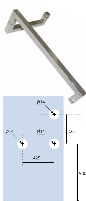
Stainless steel Shower Handle "2Π" Finishing .13
