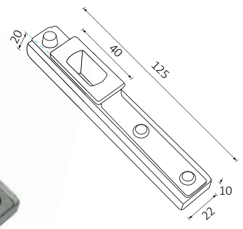
Lower Bracket FRP75 SF, Stainless Steel
