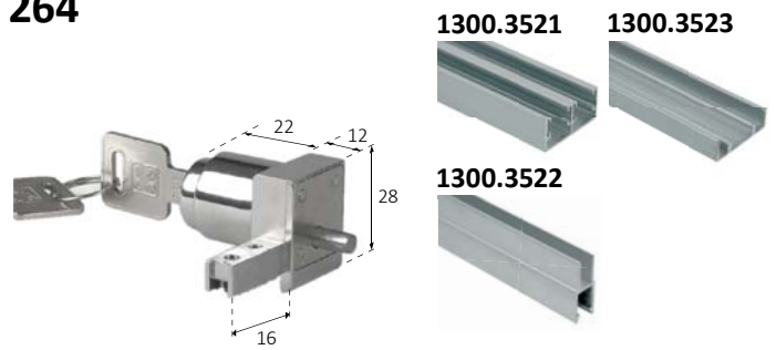
Lock for Sliding Door 5mm with profile [CODE 1300, page 78] 5mm 90 gr | Finishing .09
