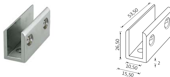
Rectangular Support
